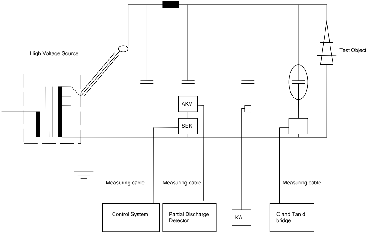
Coupling Capacitor with HV Filter Injection Capacitor Standard Capacitor
