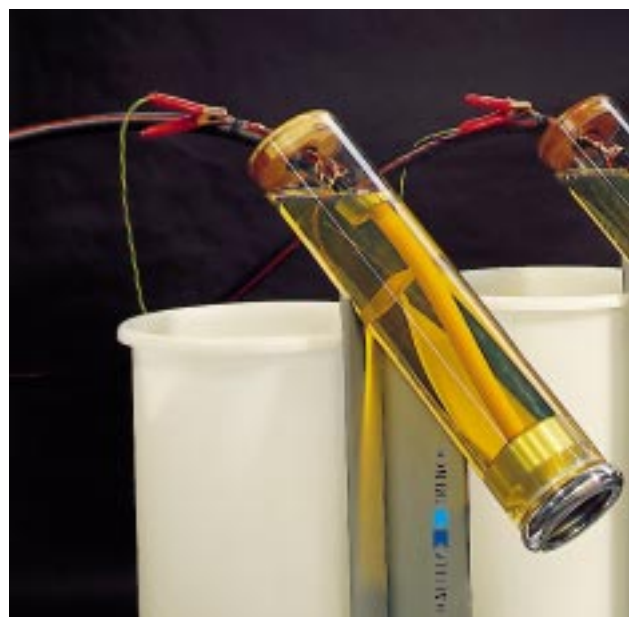
Fig. 1 Cable test termination KEV 75. 75 kV AC
