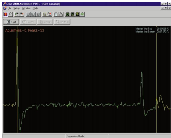
This 2452 ft cable had PD measuring 12pC in magnitude. This fault was easily detectable by adjusting the trigger level in the PDSL software program to locate lower level faults. Note that in doing so, a small amount of background noise is displayed. The Hipotronics PDSL found the fault 265 feet from the top of the cable. The customer cut around the PD site. The cable was retested and passed. Further analysis by the customer indicated that the fault was located at 265.5 feet, an accuracy of much better than .1%.
